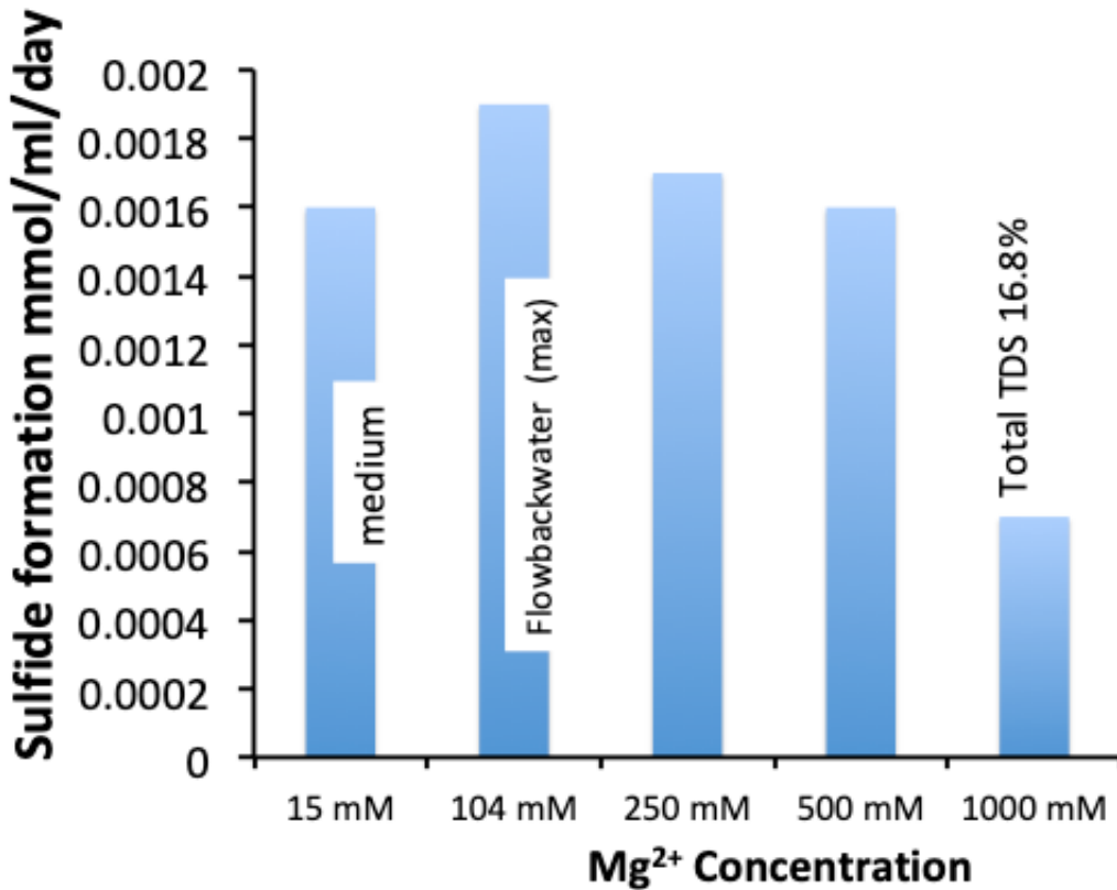
Figure 3. Rate Of Sulfide Formation By Halanaerobium , strain Lake-01 At Optimum NaCl (10%) With Various Amounts Of Mg 2+
