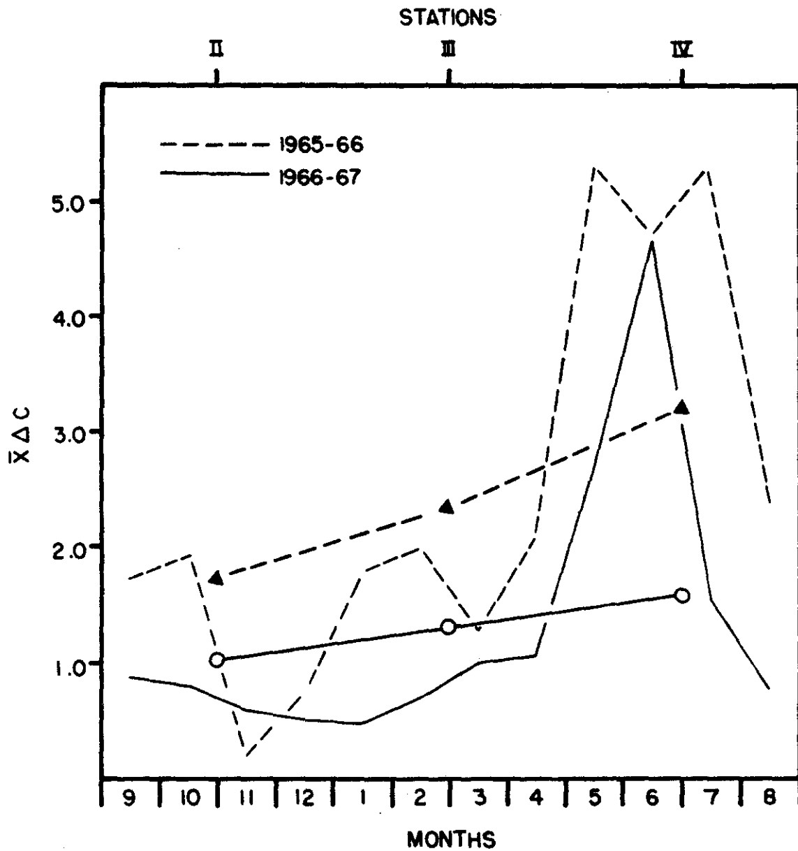
Figure 12. Comparison of monthly and station mean differences in surface and bottom temperature of Keystone Reservoir during 1965-66 and 1966-67
