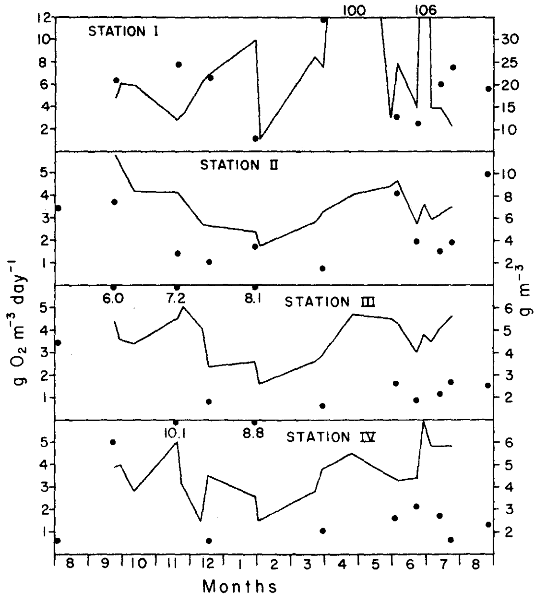
Figure 36. Temporal variation of \bar{X} concentrations of biomass (—) and \bar{R} rates of respiration (●) in the Cimarron arm during 1966-67
