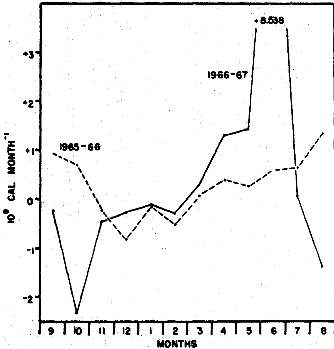
Figure 24. Comparison of monthly net gains and losses of heat due to differences in heat content of inflowing and out-flowing water during 1965-66 and 1966-67
