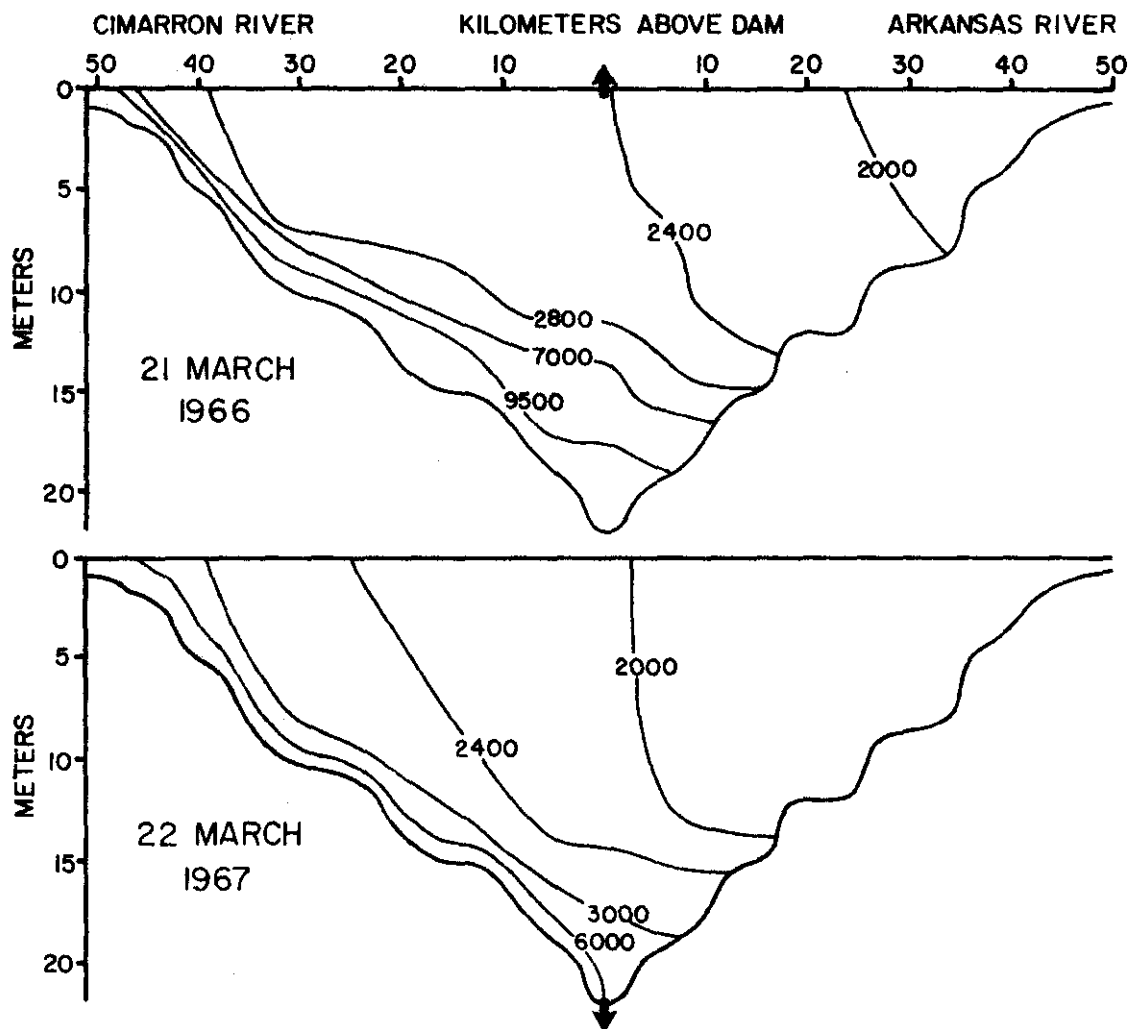
Figure 14. Isolines of conductivity ( \mu\text{mhos} ) showing density flows in Keystone Reservoir during 1966 and 1967. Arrows indicate the level at which water was being discharged through the dam.
