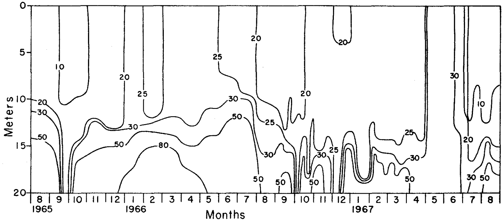
Figure 9. Isolines of conductivity ( 10^2 \mu\text{mhos} ) in Keystone Reservoir during 1965-67
