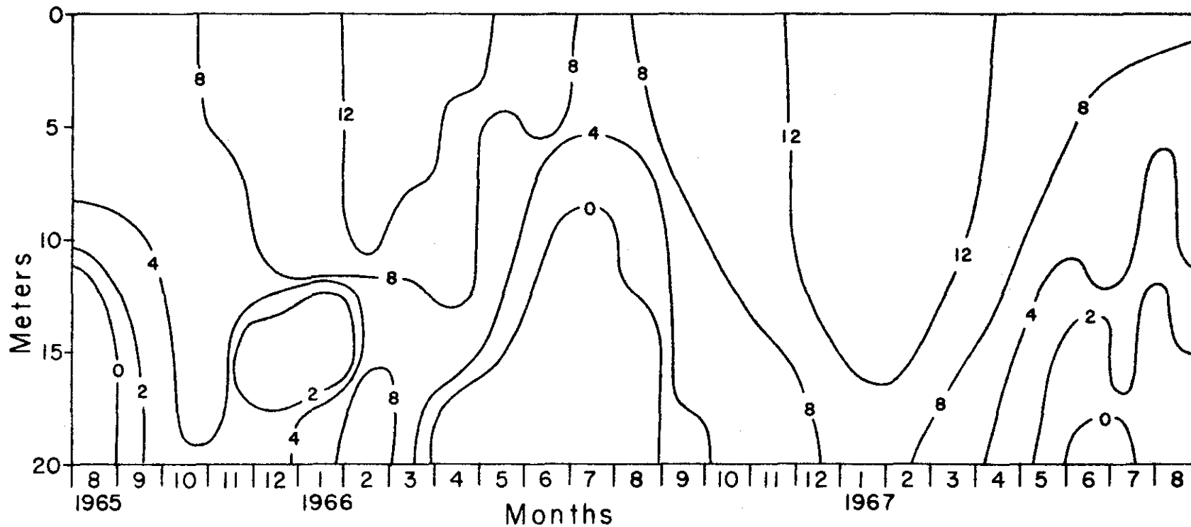
Figure 10. Isolines of dissolved oxygen concentration ( \text{g O}_2 \text{ m}^{-3} ) in Keystone Reservoir during 1965-67
