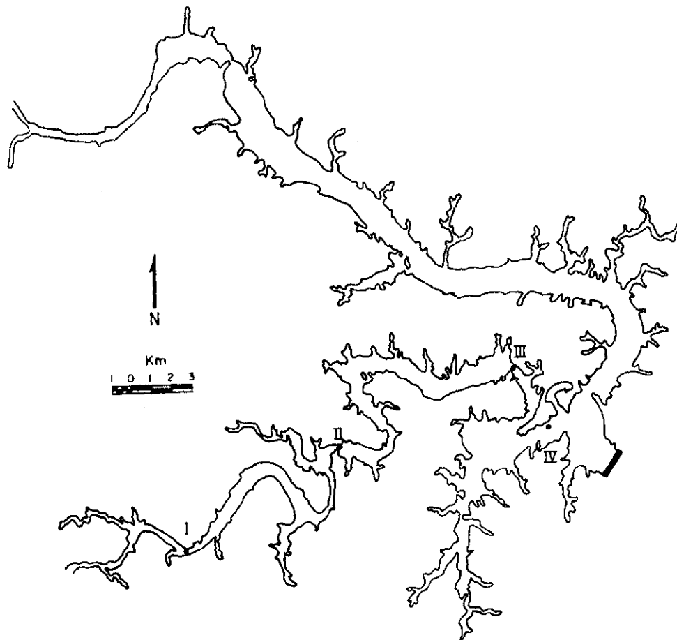
Figure 5. Keystone Reservoir, Oklahoma. Roman numerals indicate locations of sampling stations
