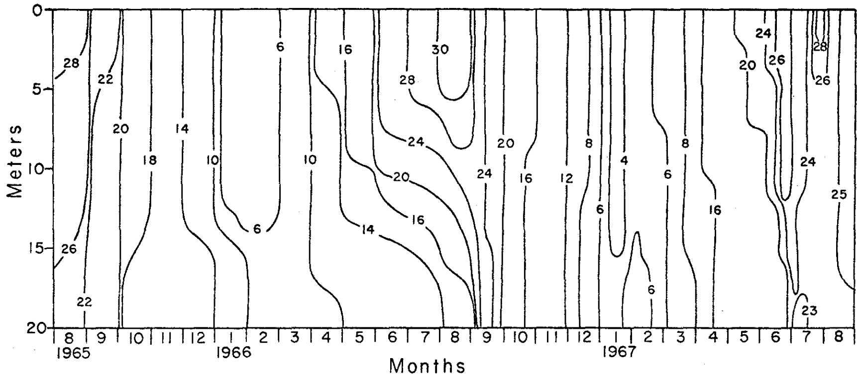
Figure 8. Isotherms of temperature (C) in Keystone Reservoir during 1965-67
