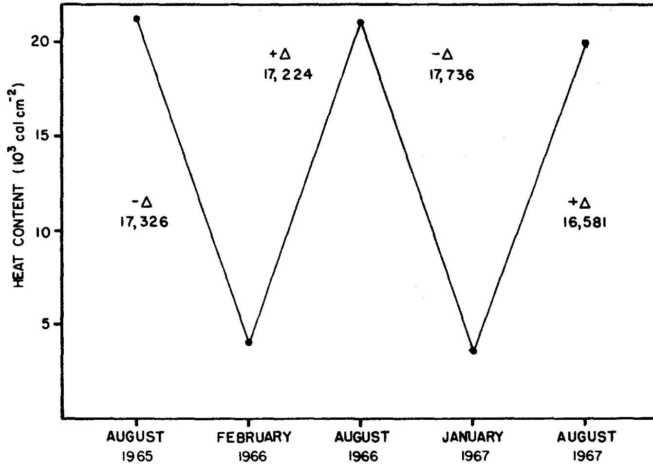
Figure 23. Minimum and maximum heat contents and Birgean heat budgets for Keystone Reservoir
