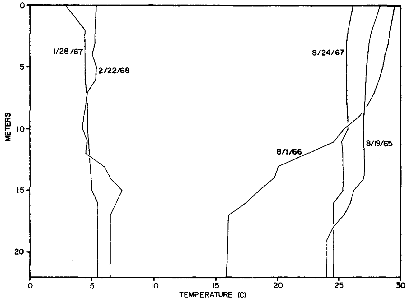
Figure 22. Average temperature profiles on dates of minimum and maximum heat content of Keystone Reservoir
