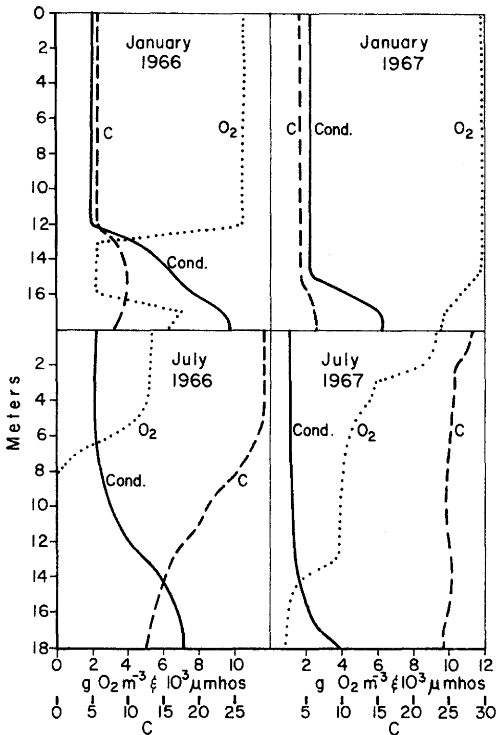
Figure 6. Winter and summer extremes of stratification at Station IV during 1966 and 1967
