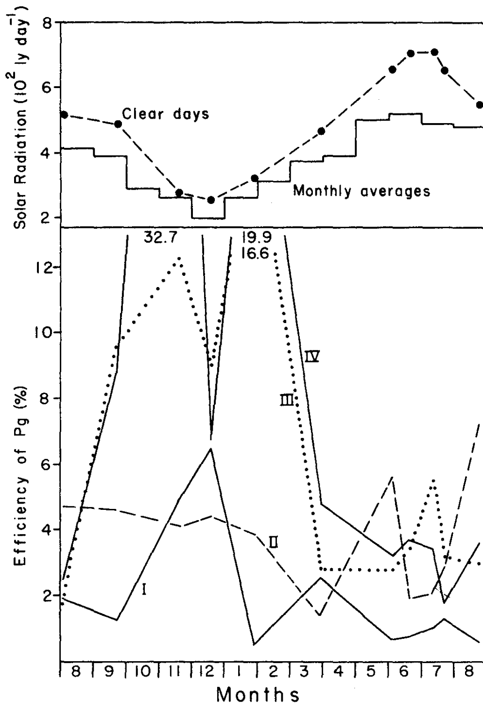
Figure 33. Comparison of solar radiation on sampling dates to monthly means of solar radiation, and spatial and temporal variations of efficiency in the Cimarron arm during 1966-67
