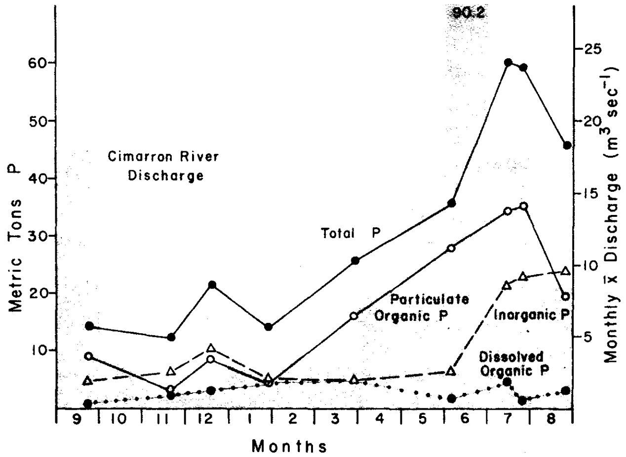
Figure 25. Relation of phosphorus content of Cimarron arm to Cimarron River discharge during 1966-67
