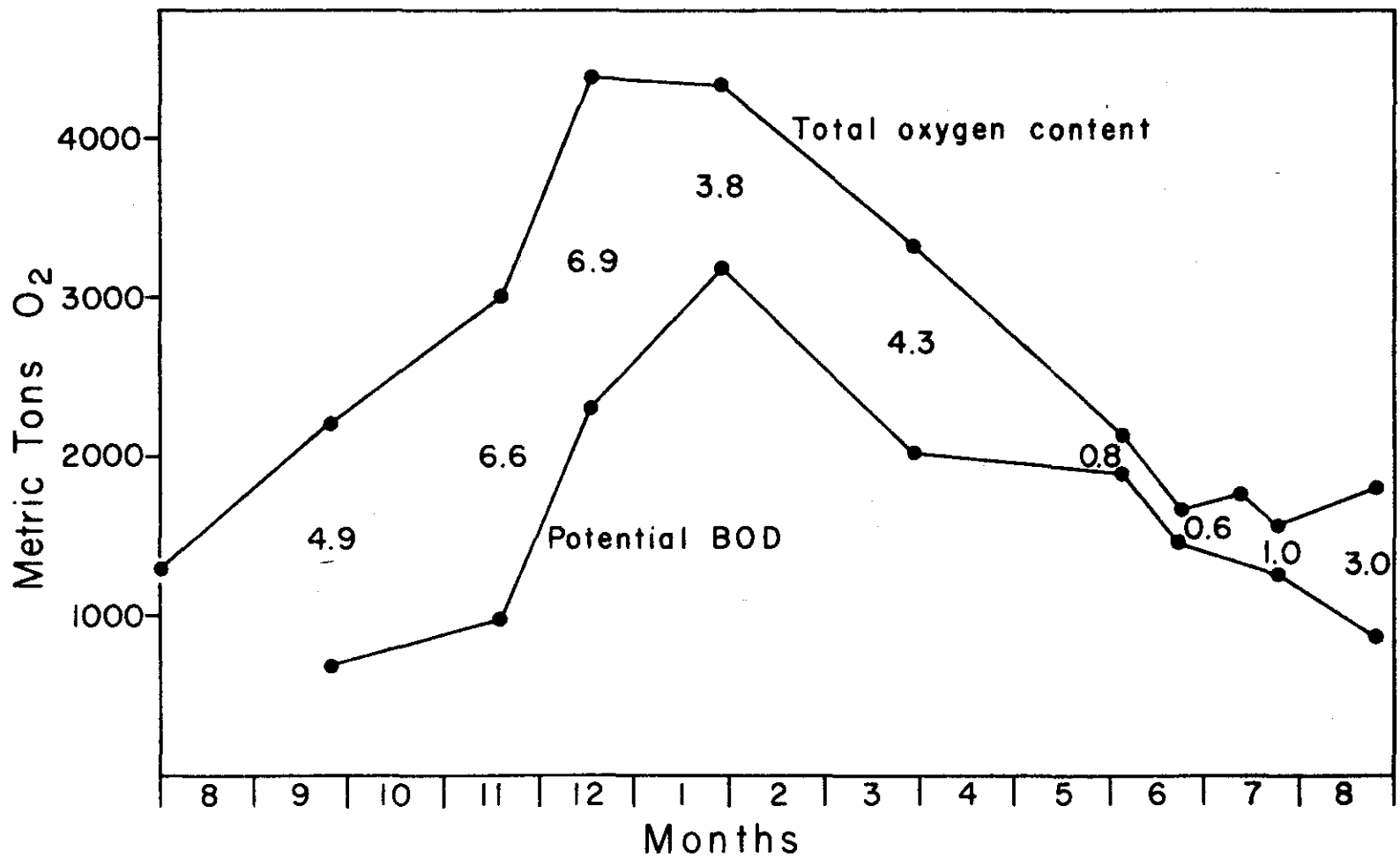
Figure 39. Comparison of total oxygen content and potential oxygen demand of the Cimarron arm on cloudless days during 1966-67. Numbers between lines are the \bar{X} \text{g O}_2 \text{ m}^{-3} of the water mass if the potential oxygen demand was exerted.
