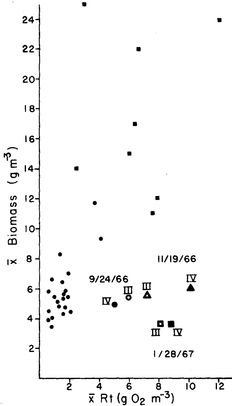
Figure 38. Relation of community respiration to biomass concentration. Large points represent data when unidentified \mu cells were the dominant form. \blacksquare = data from Station I, \bullet = data from Stations II, III, and IV.
