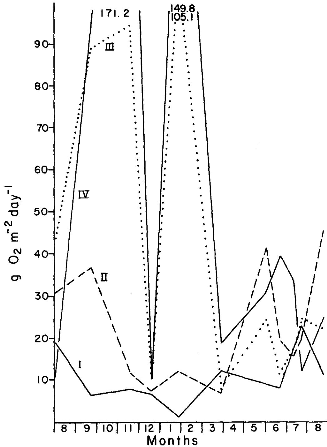
Figure 31. Temporal variation of R_t at stations in the Cimarron arm during 1966-67
