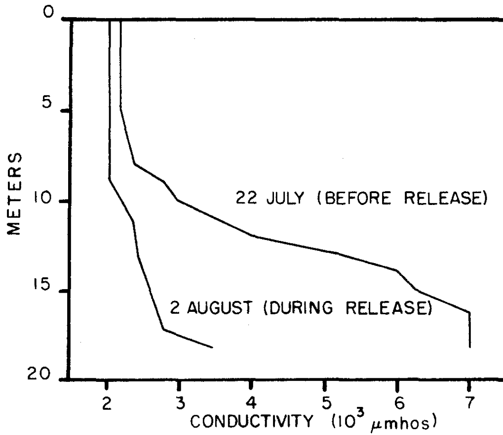
Figure 7. Effect of release of hypolimnetic water on conductivity in Keystone Reservoir, 1966
