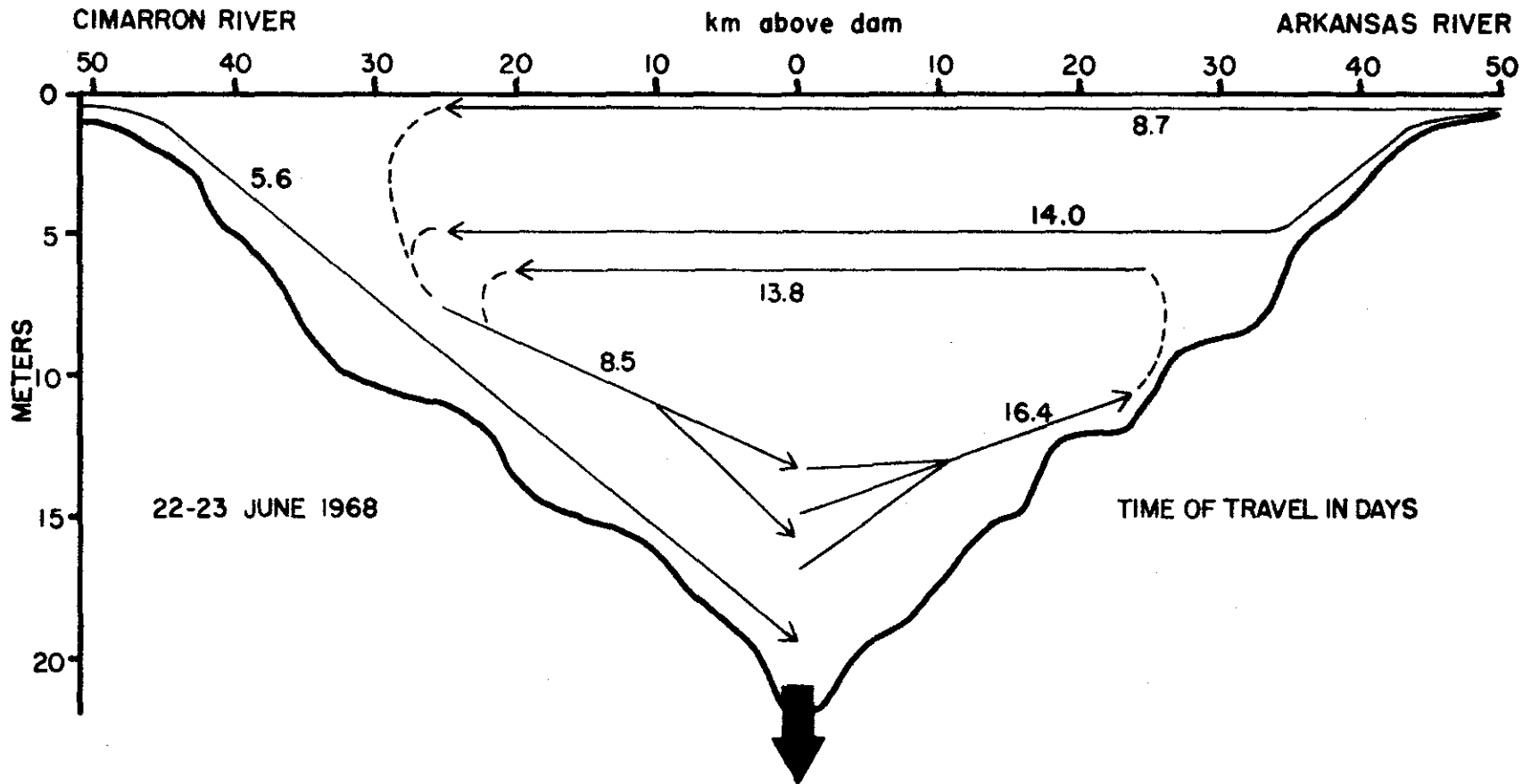
Figure 19. Estimated time of travel (days) of water masses in Keystone Reservoir assuming the physicochemical conditions present on 22-23 June 1968
