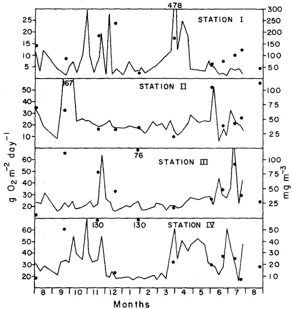
Figure 35. Temporal variation of concentrations of chlorophyll a (—) in surface water and Pg (●) in the Cimarron arm during 1966-67
