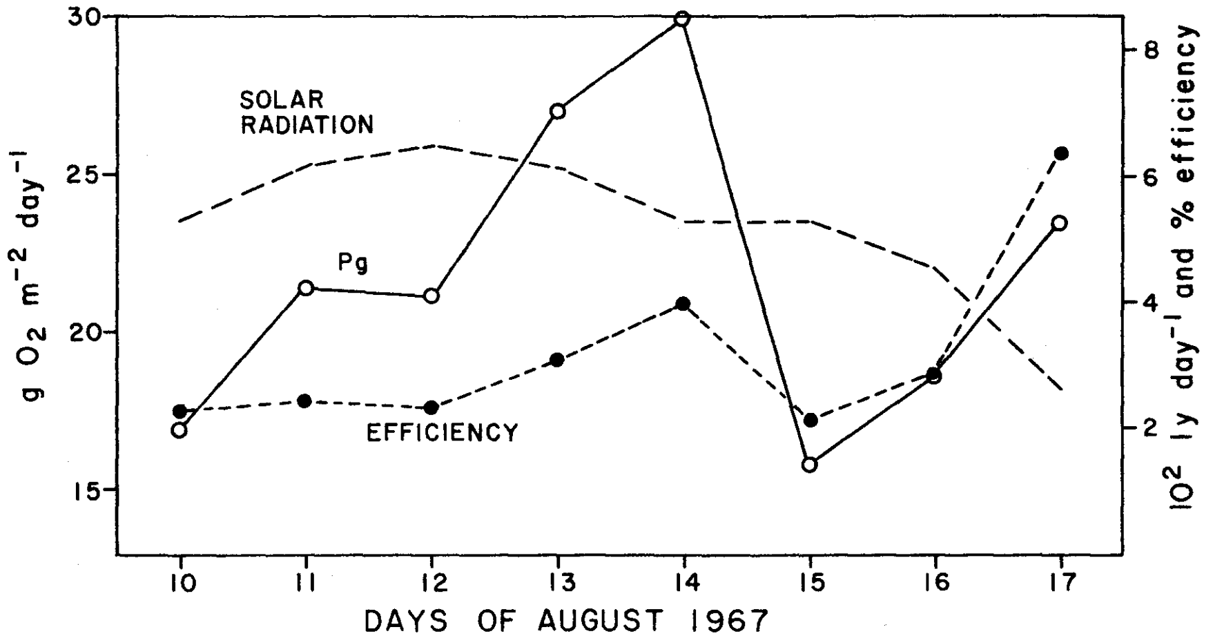
Figure 34. Relation of \text{P}_g , solar radiation, and efficiency at Station III in August 1967
