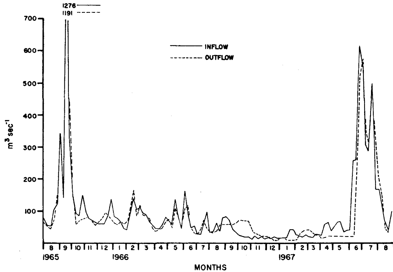
Figure 2. Temporal variations in total inflow and total outflow of Keystone Reservoir during 1965-67
