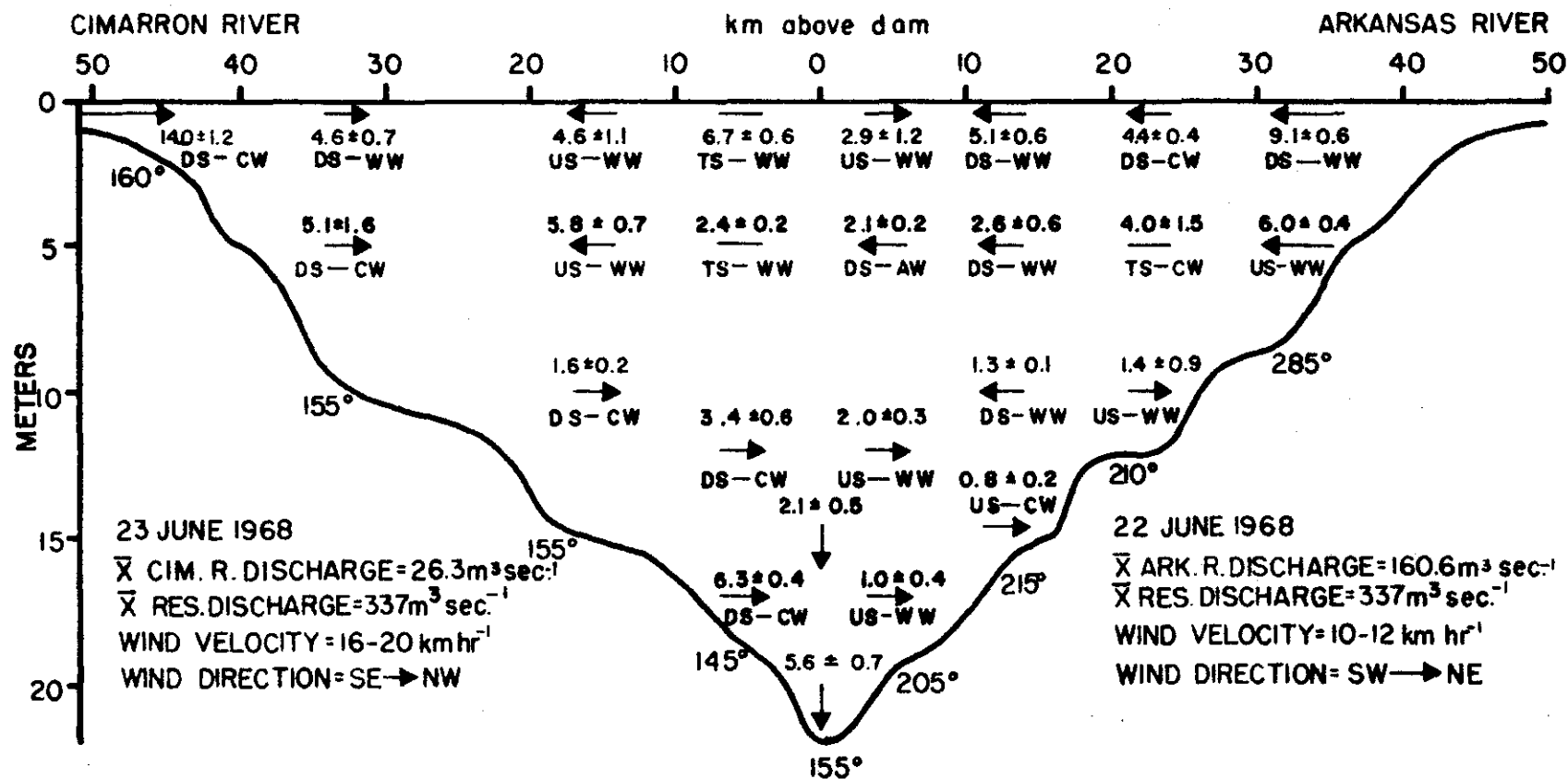
Figure 17. Speed ( \bar{x} \pm S \text{ m min}^{-1} of three observations) and direction of currents in Keystone Reservoir on 22-23 June 1968. DS = downstream, US = upstream, TS = toward shore, WW = with wind, AW = against wind, and CW = across wind. Numbers below bottom profile are the average degrees from true North from which wind was blowing during measurements at that location.
