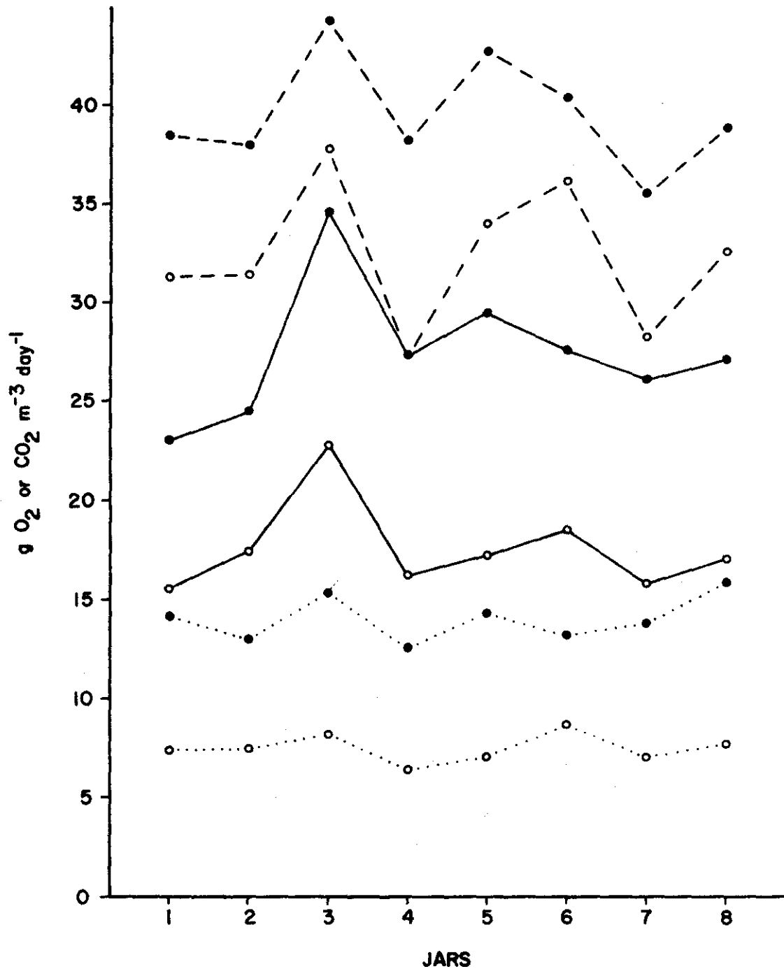
Figure 28. Comparison of the rates of community metabolism in eight laboratory microcosms containing water from Keystone Reservoir as measured by the pH- CO_2 curve method (---), O_2 curve method (—), and light and dark bottle method (····). ● = \bar{X} gross primary productivity, and ○ = \bar{X} total community respiration (2 replicate measurements per jar).
