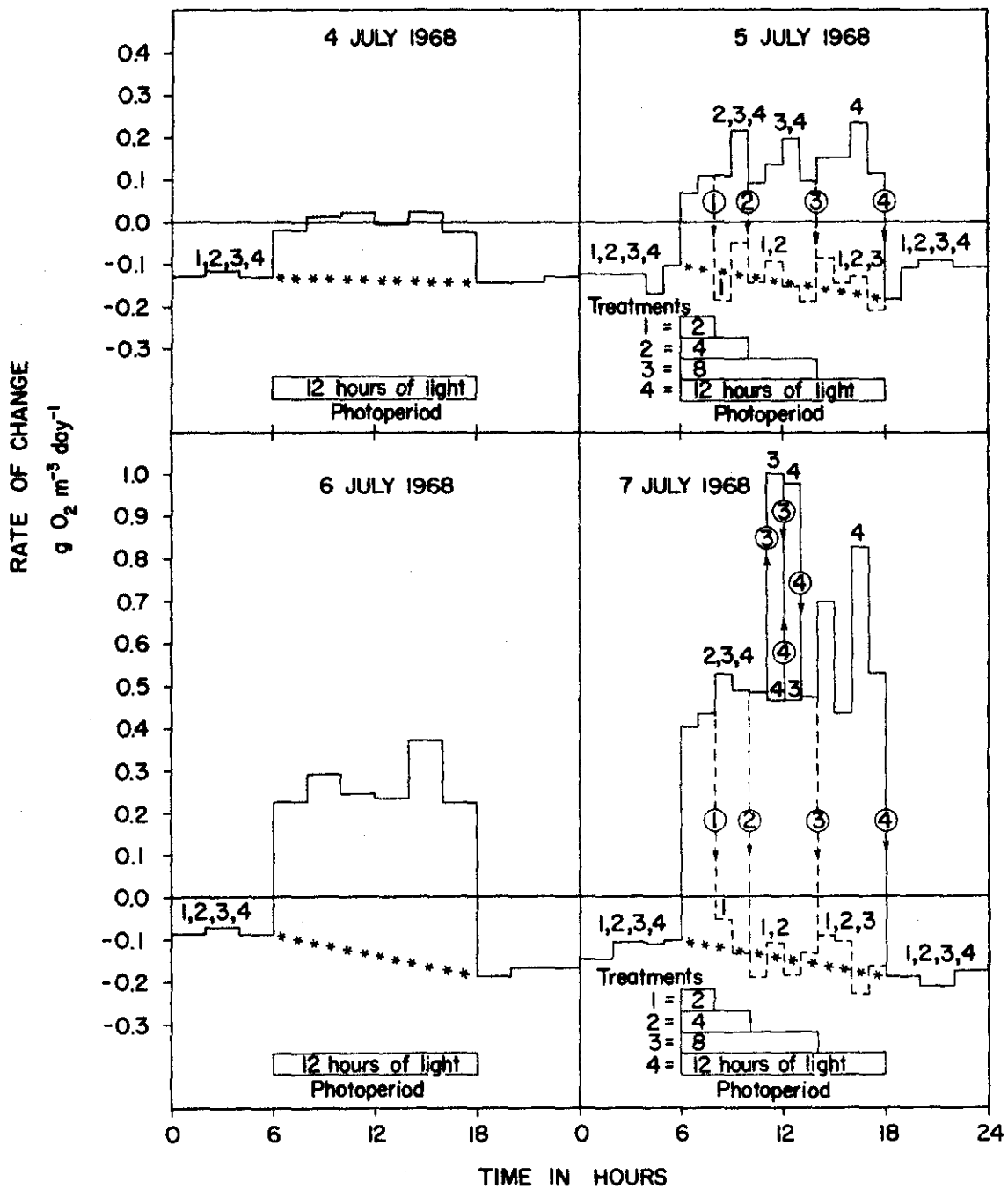
Figure 27. Effect of a varied photoperiod on the rate-of-change of oxygen in eight laboratory microcosms during the early stages of succession. --- = negative rate-of-change observed after light was extinguished in treatments receiving a photoperiod shorter than 12 hours. *** = hypothetical daytime respiration line of treatments receiving a 12-hr photoperiod. When treatment \bar{X} rates-of-change were not significantly different ( \alpha = 0.05 ), \bar{x} is represented by a single line. Numbers on the rate-of-change line indicate which treatments are represented by that segment of the line.
