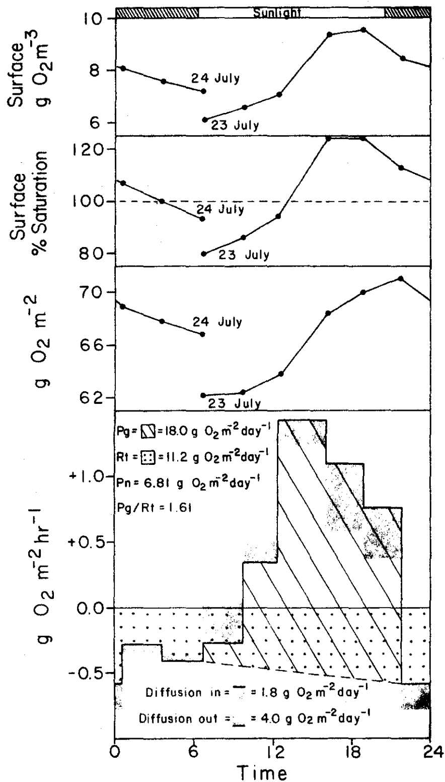
Figure 26. Community metabolism and atmospheric reaeration at Station IV, Keystone Reservoir, 23-24 July 1967, as calculated by the O_2 curve method ( k = 1.98 )
