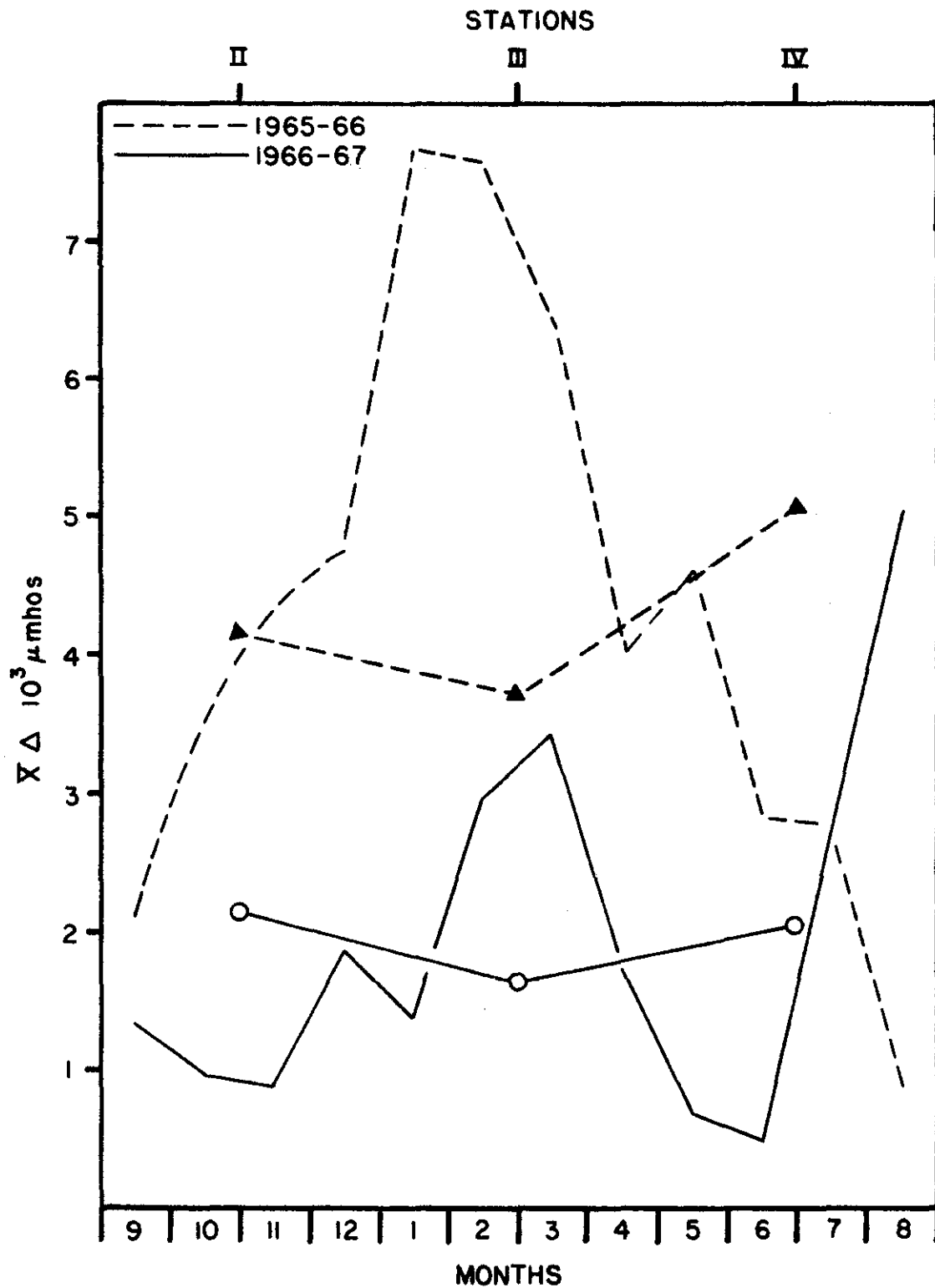
Figure 13. Comparison of monthly and station mean differences in surface and bottom conductivity of Keystone Reservoir during 1965-66 and 1966-67
