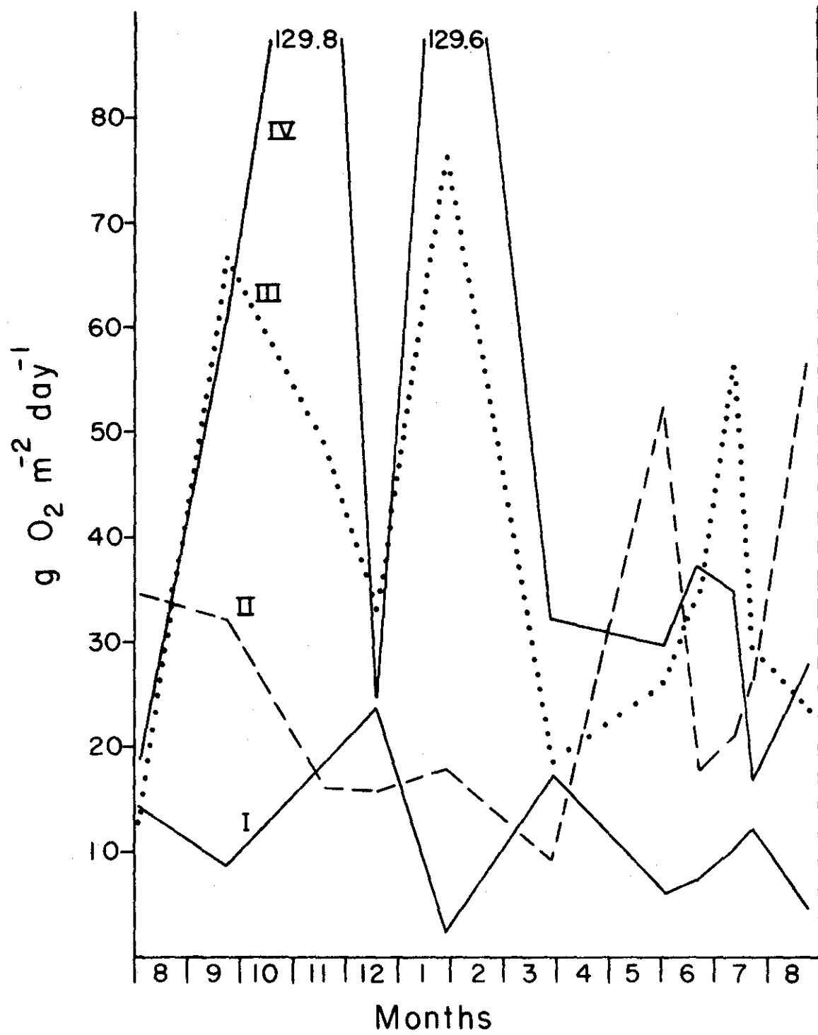
Figure 30. Temporal variation of Pg at stations in the Cimarron arm during 1966-67
