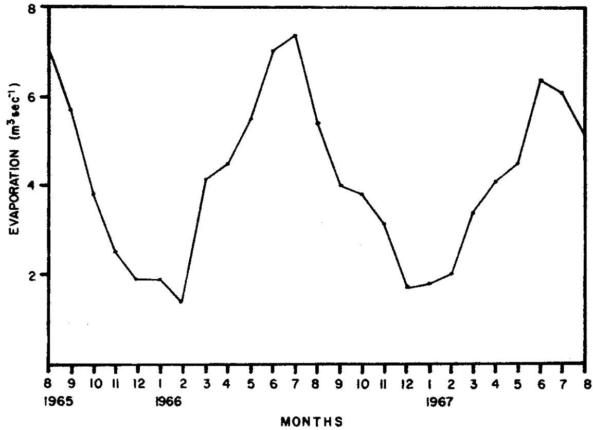
Figure 4. Temporal variations in the monthly average rate of evaporation for Keystone Reservoir derived from records of the U. S. Army Corps of Engineers
