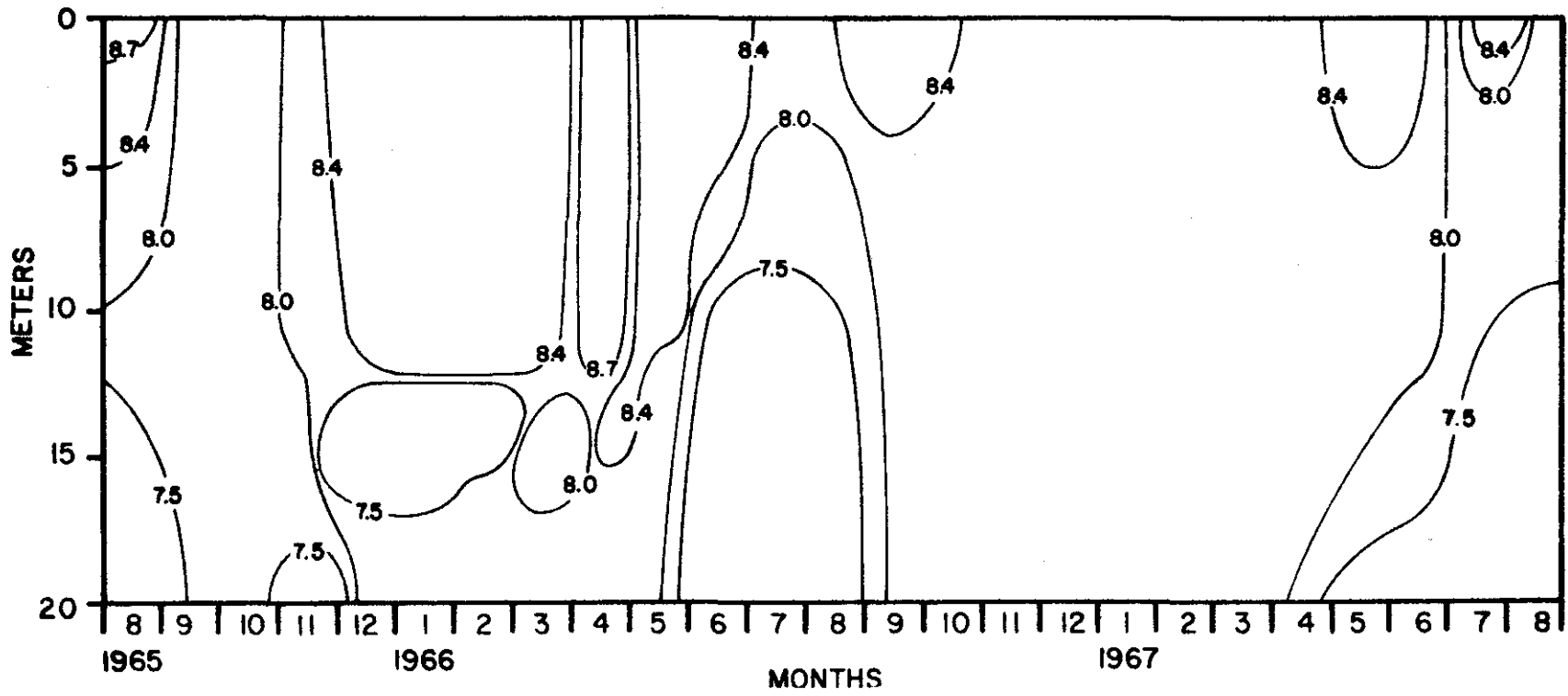
Figure 11. Isolines of pH in Keystone Reservoir during 1965-67
