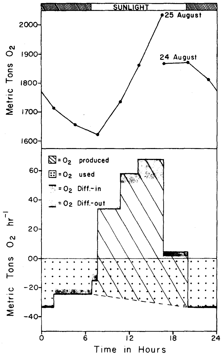
Figure 40. Analysis of oxygen budget of Cimarron arm, 24-25 August 1967, by O 2 curve method. See Table XXVI for calculations.
