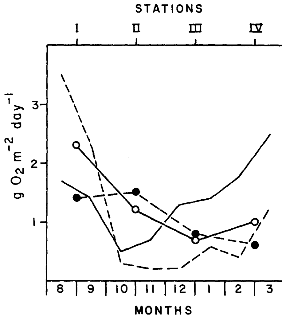
Figure 29. Annual station means ( \circ , \bullet ) and monthly means (—, —) of gross productivity (—, —) and respiration (---, ---) in the euphotic zone of Keystone Reservoir during 1965-66 as measured by the light and dark bottle method
