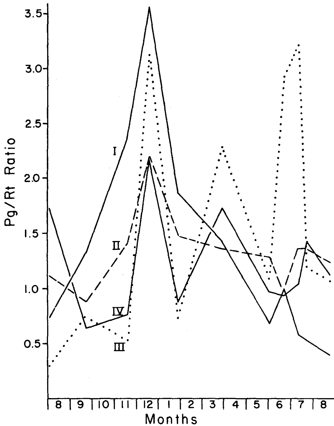
Figure 32. Temporal variation of Pg/Rt ratios at stations in the Cimarron arm during 1966-67
