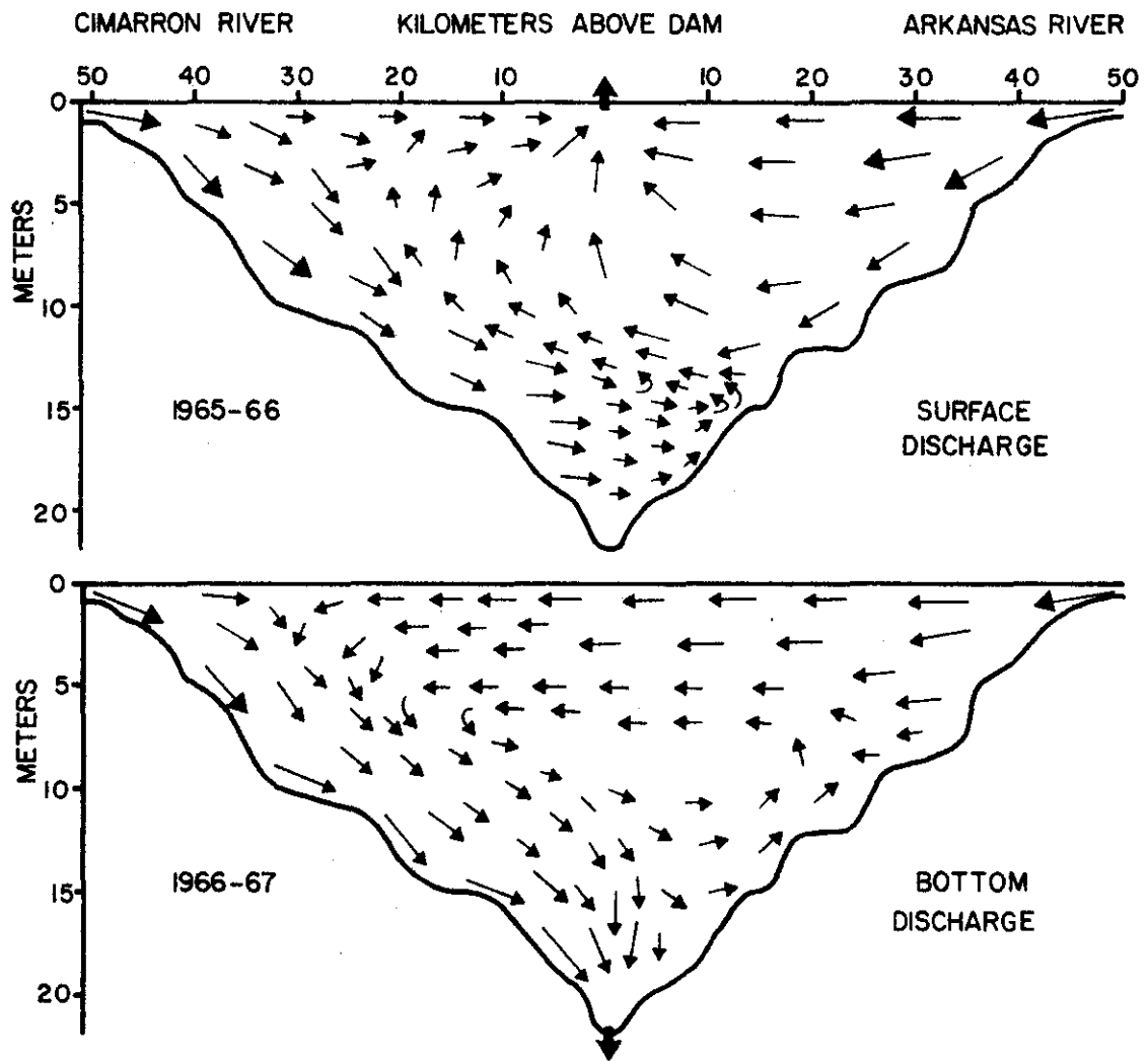
Figure 18. Effects of the level of reservoir discharge on circulation patterns in Keystone Reservoir. Relative speed of flows, which was derived from current measurements, is indicated by the size of arrows. General direction of flows was derived from current measurements, isolines of conductivity, and distribution of Cl/SO_4 ratios. Direction of flows above 5 m of depth often was modified by wind action.
