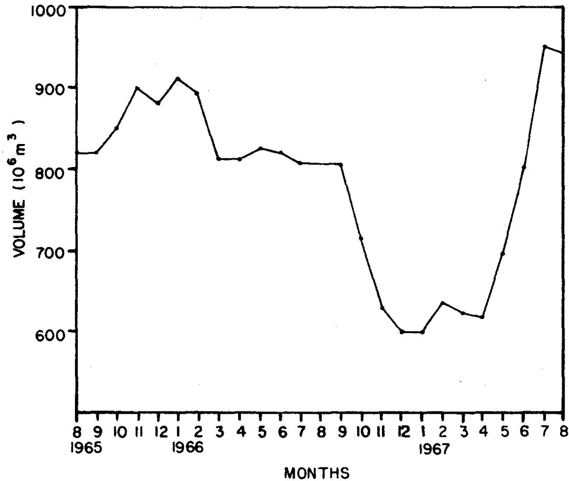
Figure 3. Temporal variations in the monthly average volume of Keystone Reservoir derived from records of the U. S. Army Corps of Engineers
