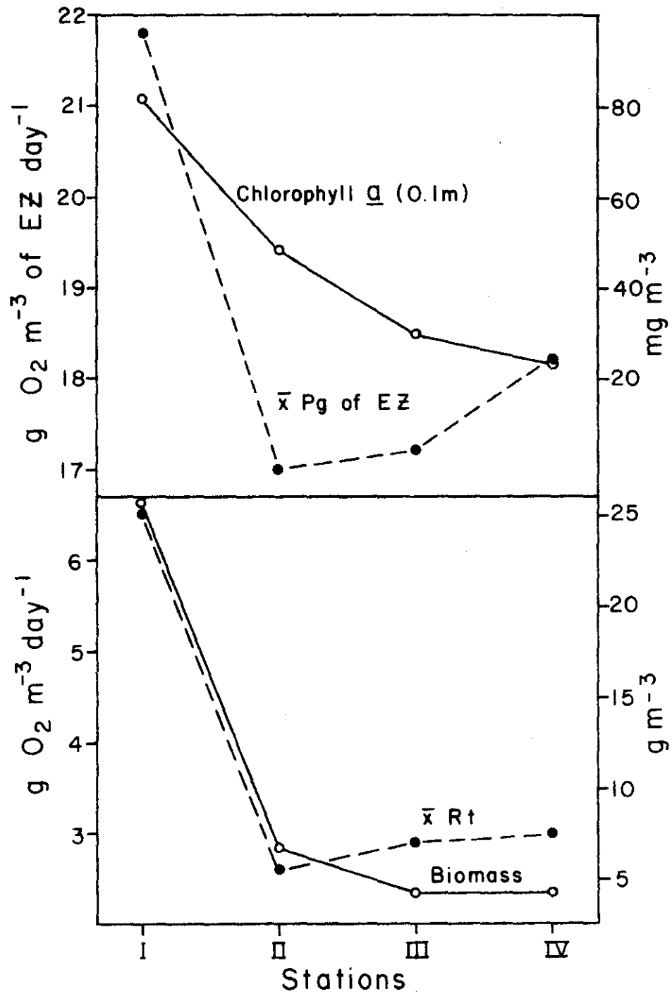
Figure 37. Spatial variations in annual mean plankton structure and function in the Cimarron arm during 1966-67
