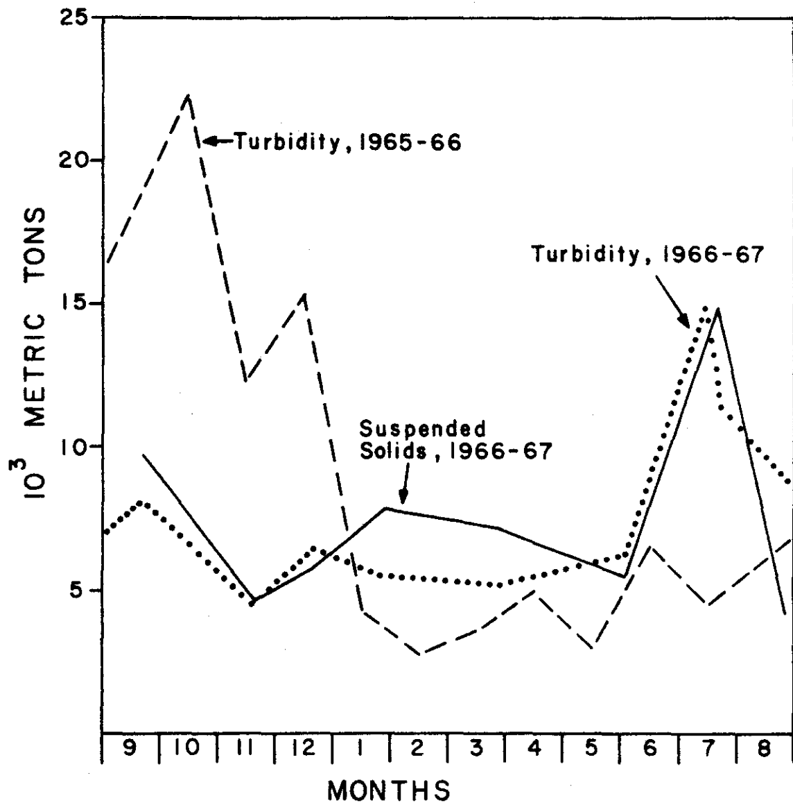
Figure 21. Comparison of turbidity and suspended solids content of the Cimarron arm during 1965-66 and 1966-67
