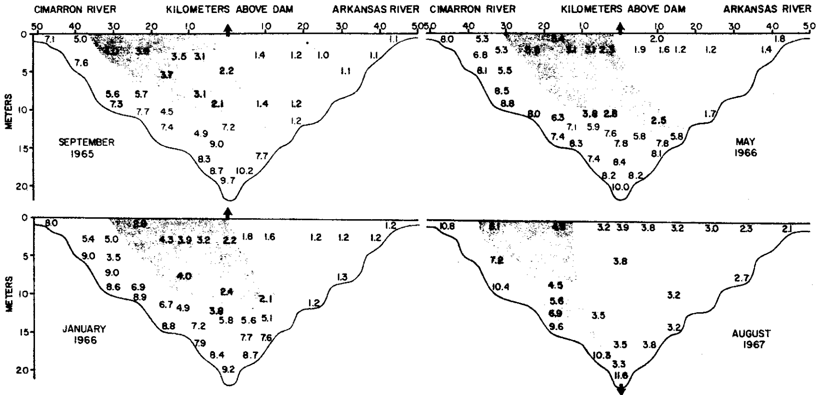
Figure 15. Chloride/sulfate ratios in Keystone Reservoir during 1965-67. High ratios identify water primarily of Cimarron River origin while low ratios identify water contributed by the Arkansas River. Shaded areas indicate zones of mixing.
