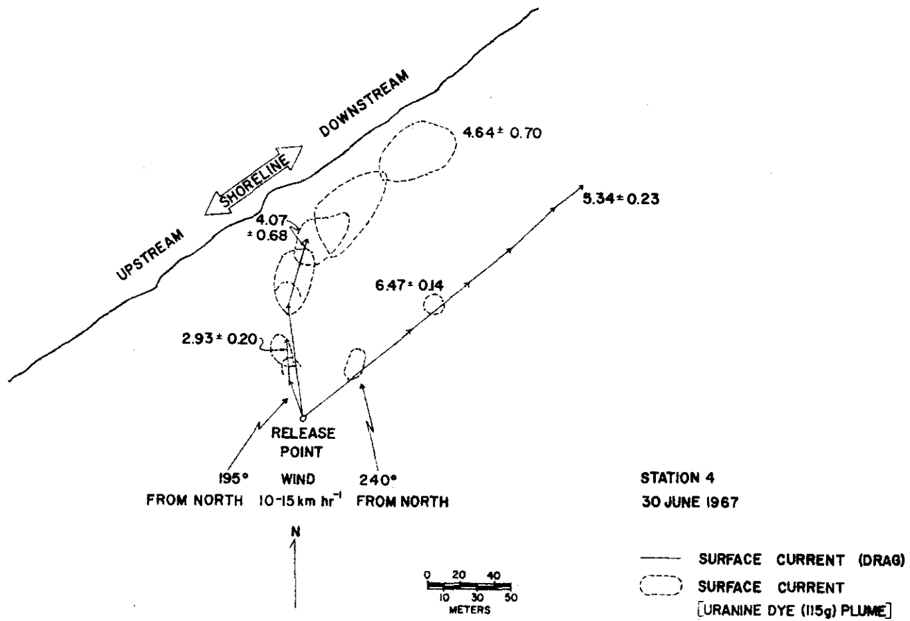
Figure 16. Comparison of the speed ( \text{m min}^{-1} ) and direction of surface currents as estimated by the free-drag and dye plume methods
