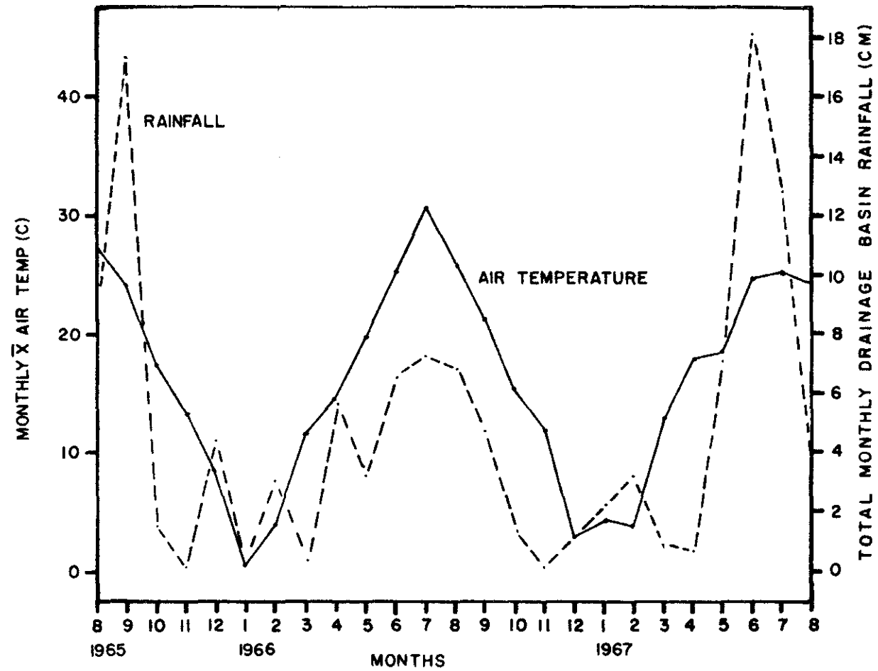
Figure 1. Drainage basin rainfall and air temperature during 1965-67 from records of U. S. Army Corps of Engineers and U. S. Weather Bureau
