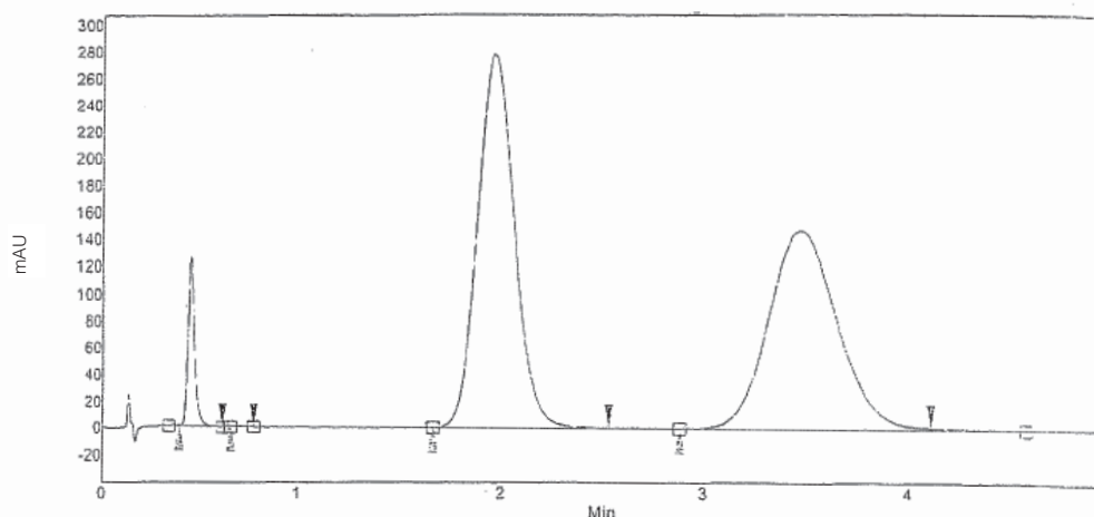
Figure 4. Chromatogram for the original mixture of enantiomers.
