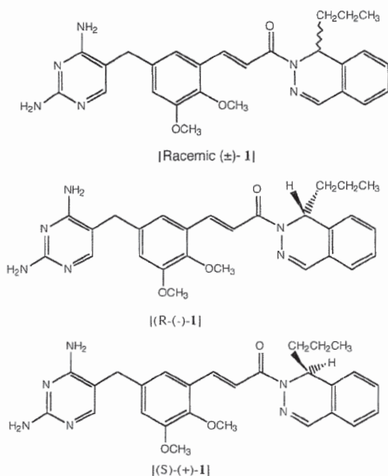
Figure 1. The structures of racemic (±)-1, (R)-(-)-1, and (S)-(+)-1.
