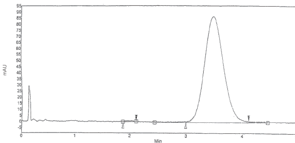
Figure 2. Chromatogram for (R)-(-)-1.
