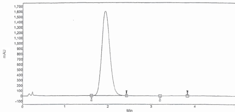
Figure 3. Chromatogram for (S)-(+)-1.
