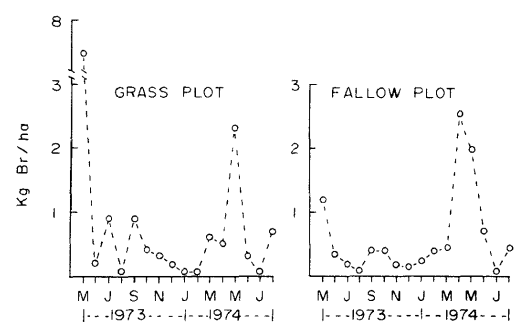
FIGURE 2. Amounts of bromide lost in runoff from grass and fallow plots from May 1973 through August 1974.
